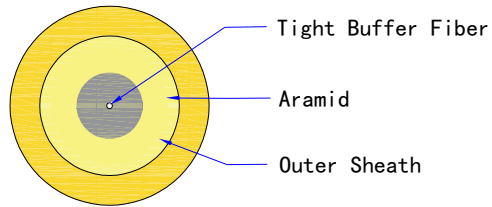
Single core cable
